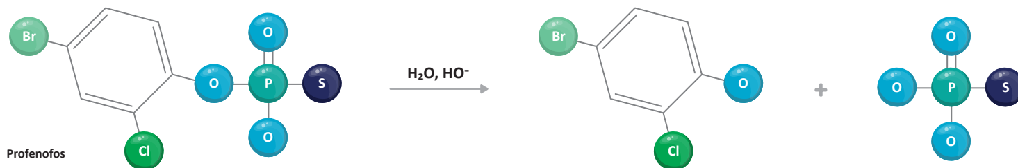
Figure 1: The Hydrolysis of Profenofos.
